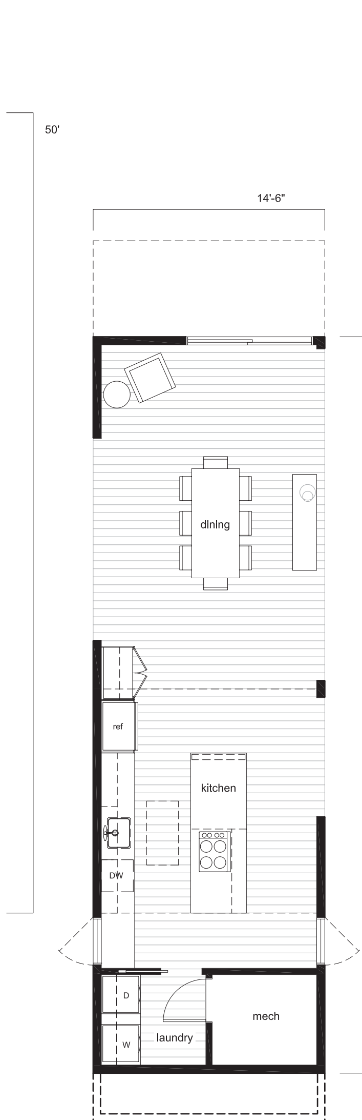
A total area: 667sf
